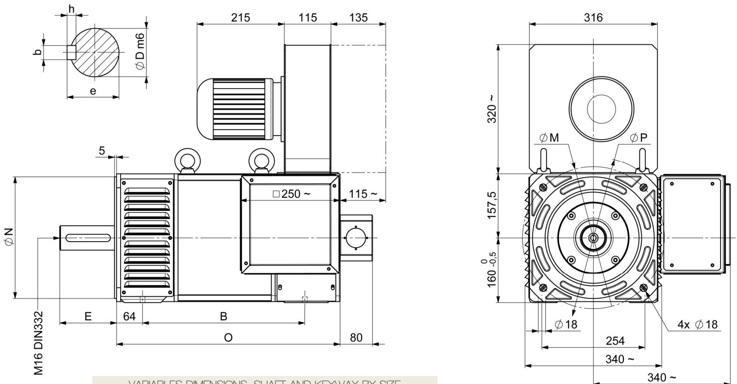
VARIABLES DIMENSIONS, SHAFT AND KEYWAY BY SIZE
