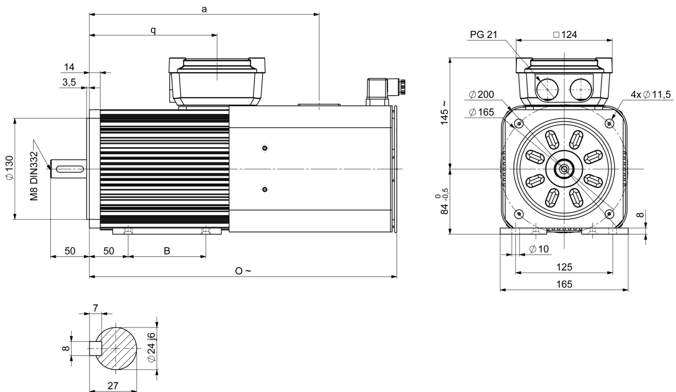
VARIABLES DIMENSIONS BY SIZE
